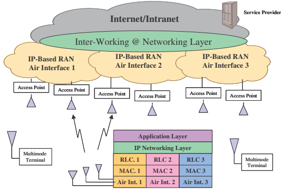
Figure 3: Short Term Architectural Perspective
