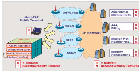
Figure 9: E 2 R Prototyping Environment
