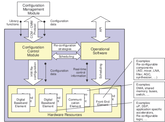
Figure 7: Radio Modem Reconfigurability Research
