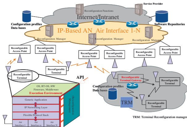
Figure 4: E 2 R Architectural Vision
